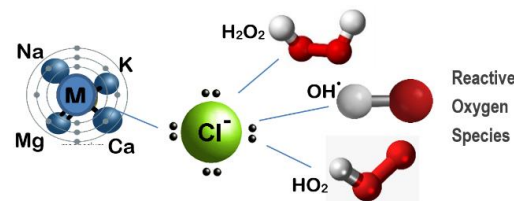
Figure 1 — Proposed structures for mineral oxychlorides and the reactive oxygen species they release in water.
