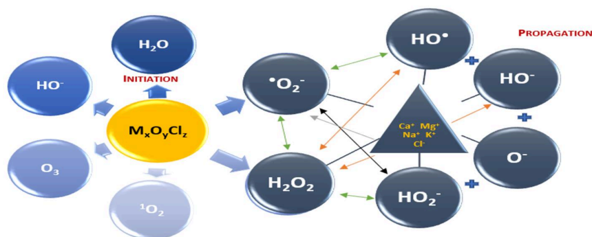
Figure 2 — Chain-reaction phases of the mineral oxychloride reagent: initiation, propagation, and termination. The reaction is autocatalyzed by the inherent mineral catalysts ( \text{Ca}^{2+} , \text{Mg}^{2+} , \text{Na}^+ , \text{K}^+ , \text{Cl}^- ).
